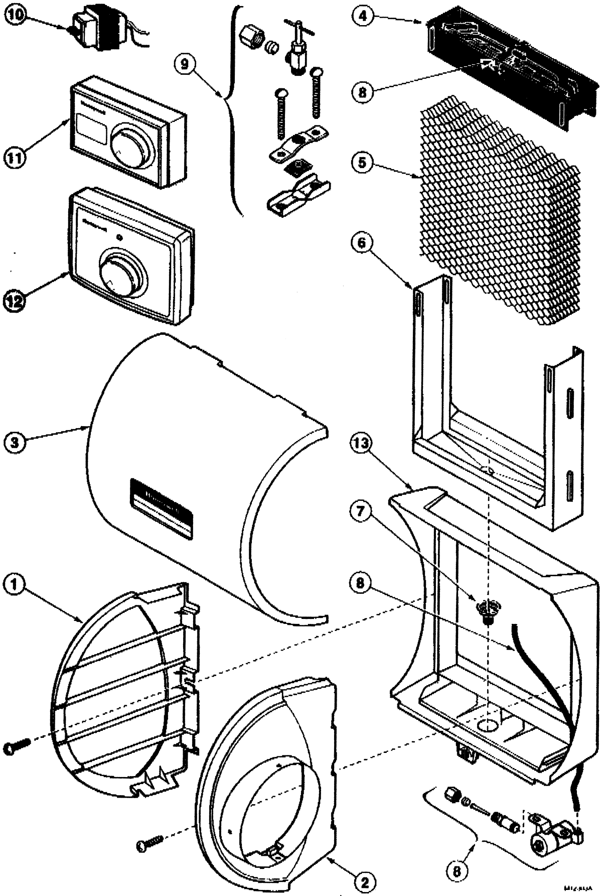
HE260 EXPLODED VIEW. PART NUMBERS ARE KEYED TO PARTS LIST.
